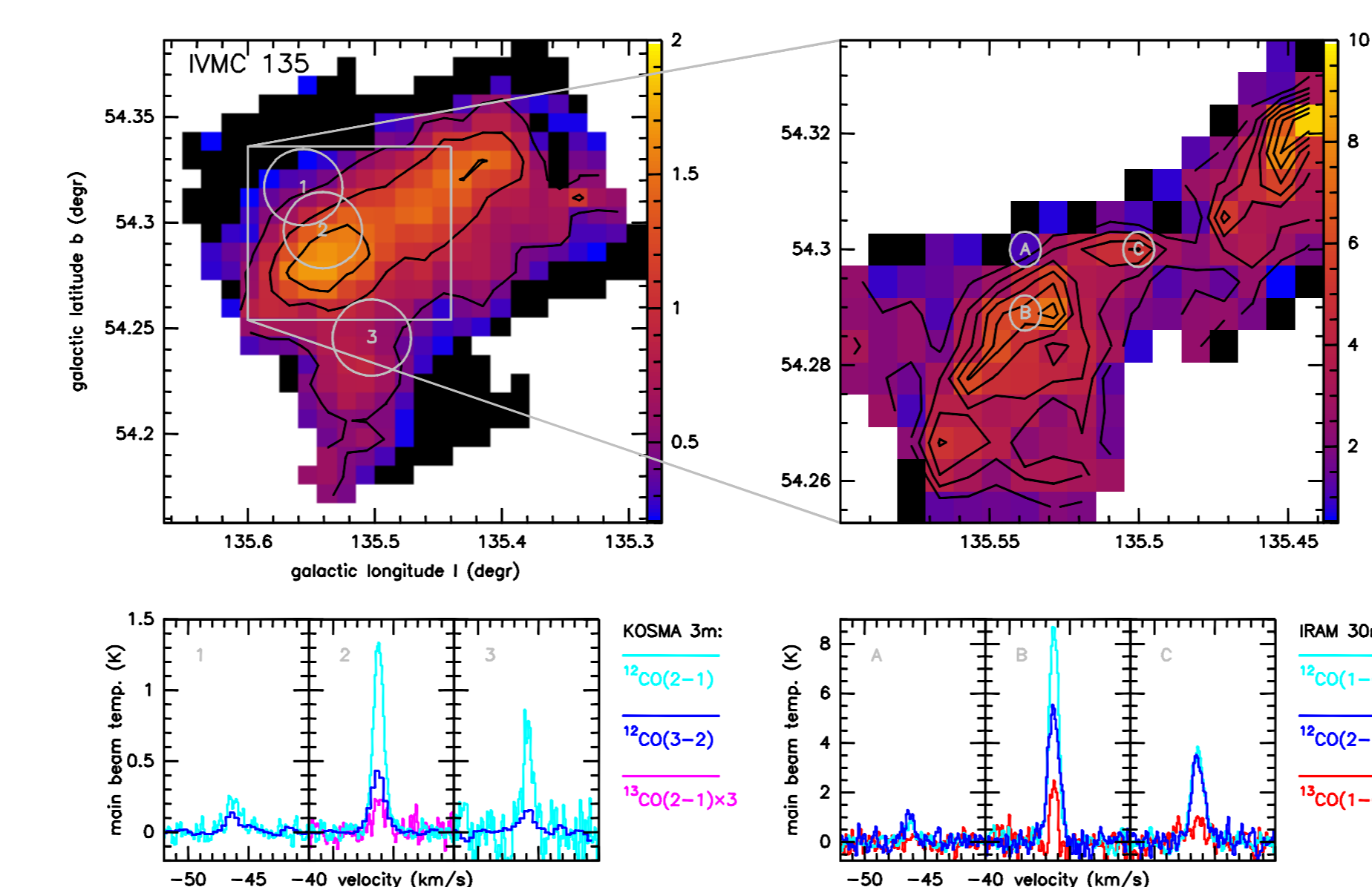
Fig. 3: IVMC135: line-integrated intensity map for the ^{12}\text{CO} J=2-1 observations made with the KOSMA 3m telescope (top left panel) and Pico Veleta 30m telescope (top right). Line profiles are shown for three selected positions in each map. The position are marked by numbers (letters) in the upper panels, with the circle indicating the main beam FWHM of the telescope.
